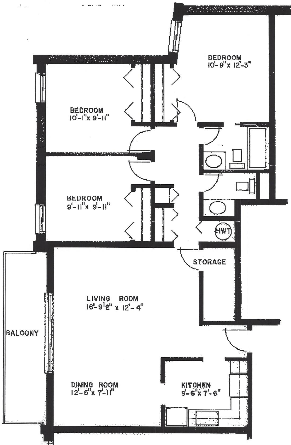
TYP. THREE BEDROOM END UNIT (FIRST FLOOR ONLY) BAYVIEW APARTMENT (1155.7 SQ. FT.)
